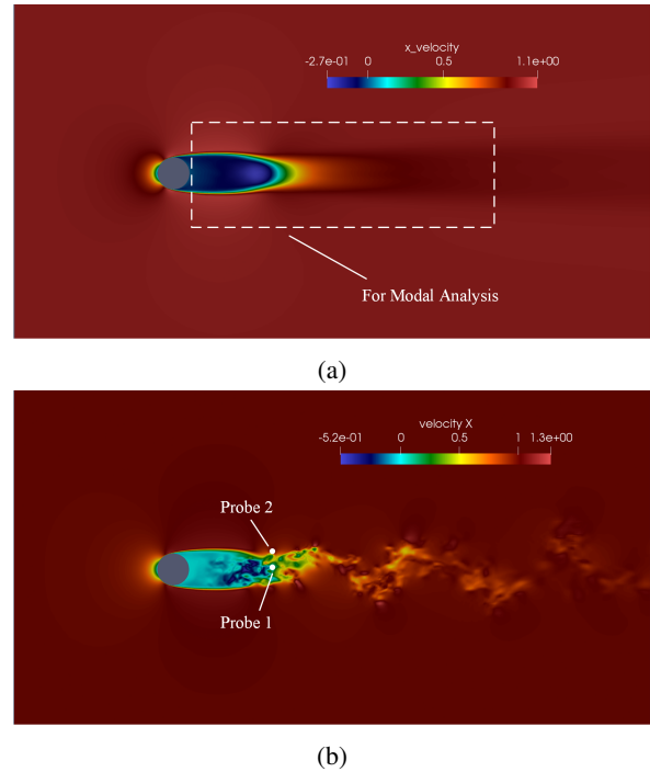
Figure 3: Temporally-averaged (top) and instantaneous (bottom) streamwise velocity contours on the plane z = 0 .
