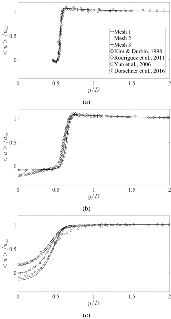
Figure 2: Time-averaged streamwise velocity profiles at (a) x = 0.2D , (b) x = 1.6D , (c) x = 3D , in comparison with available data. The center of the sphere is at (0,0,0) .
