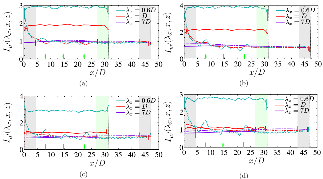
FIG. 17. Streamwise intermittency function of the WT array and the neutral ABL for (a), (c) u velocity, I_{u'}(\lambda_x, x, z) , and (b), (d) w velocity, I_{w'}(\lambda_x, x, z) . Both intermittency functions are normalized by the streamwise-averaged energy spectra of the WT array. (a), (b) z = 0.125D , inner layer; (c), (d) z = 4.375D , outer layer. Lines, color marks, and gray or green patches, same as in Fig. 16.
