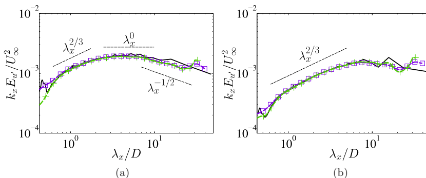
FIG. 5. Validation of the wavelet transform: comparison of a streamwise-integrated spectrum, k_x \tilde{E}_u(\lambda_x)/U_\infty^2 , between Morlet and Morse wavelets and a Fourier transform. (a) z = 0.125D , inner layer; (b) z = z_h + D/2 , top tip of the rotor. Green +, Morlet wavelet spectra; violet \square , Morse wavelet spectra; solid black, Fourier spectra.
