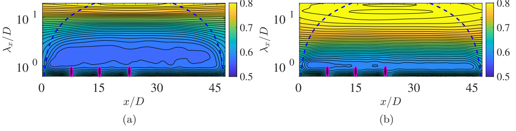
FIG. 11. Wavelet spectral vertical coherence of streamwise velocity u' (left) and wall-normal velocity w' (right) in the outer layer, \rho_{\mathcal{W}\psi}[u'_i, u'_j](k_x, x, z, z') . (a) u' coherence and (b) w' coherence. z = z_o , z' = z_o + D/2 , z_o = 4.125D . Black and pink markers, streamwise location of the turbine rows; blue dashed line, boundary of the COI.
