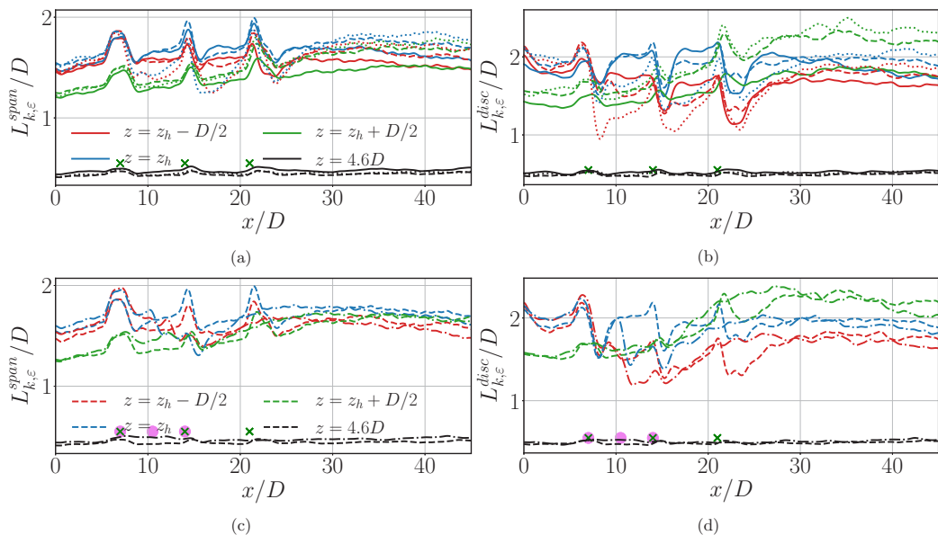
FIG. 15. Mixing length scales [Eqs. (A1) and (A2)] at different heights for the different cases simulated as in Table III. Solid lines, \lambda_R^3 s_{x,7D} ; dashed lines, \lambda_R^5 s_{x,7D} ; dotted lines, \lambda_R^8 s_{x,7D} ; dash-dotted lines, \lambda_R^5 s_{x,3.5D} . Left: Spanwise-averaged correlation length scales. Right: Disk-averaged correlation length scales. Green crosses, wind turbine locations with s_x = 7D ; pink circles, wind turbine locations with s_x = 3.5D .
