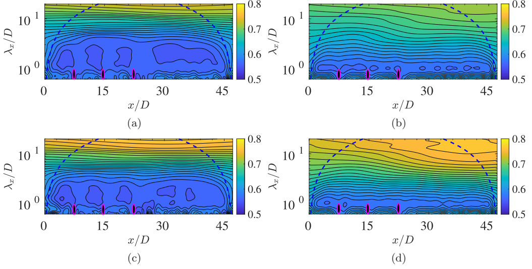
FIG. 10. Wavelet spectral vertical coherence of streamwise velocity u' (left) and wall-normal velocity w' (right) in the rotor region, \rho_{\mathcal{W}\psi}[u'_i, u'_j](k_x, x, z, z') . (a), (c) u' coherence. (b), (d) w' coherence. (a), (b) z = z_h , z' = z_h - D/2 ; (c), (d) z = z_h , z' = z_h + D/2 . Black and pink markers, streamwise location of the turbine rows. Blue dashed line, boundary of the COI.
