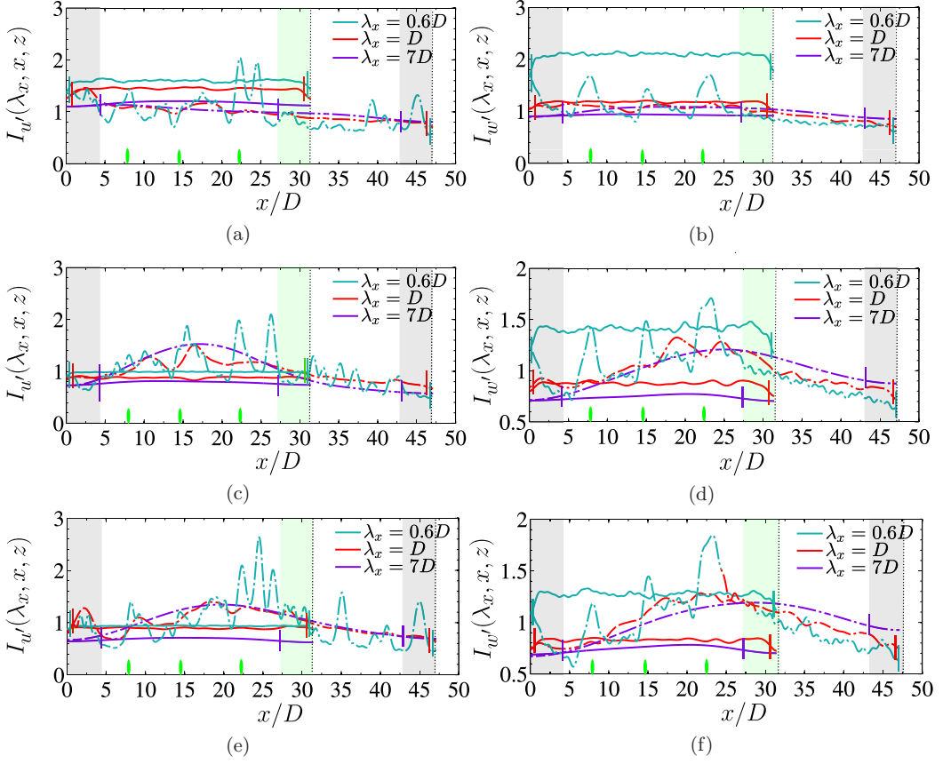
FIG. 16. Streamwise intermittency function of the WT array and the neutral ABL for (a), (c), (e) u velocity, I_{u'}(\lambda_x, x, z) , and (b), (d), (f) w velocity, I_{w'}(\lambda_x, x, z) . Both intermittency functions are normalized by the streamwise-averaged energy. (a), (b) z = z_h - D/2 , bottom tip of the rotor; (c), (d) z = z_h , hub height of the rotor; (e), (f) z = z_h + D/2 , top tip of the rotor. Solid lines, ABL domain; dash-dotted lines, WT domain. Color marks, boundaries of the COI for the WT and ABL domains. Gray or green patches, regions inside the COI of the wavelet with the maximum wavelength considered, \lambda_x = 12D for the WT and ABL domains, respectively.
