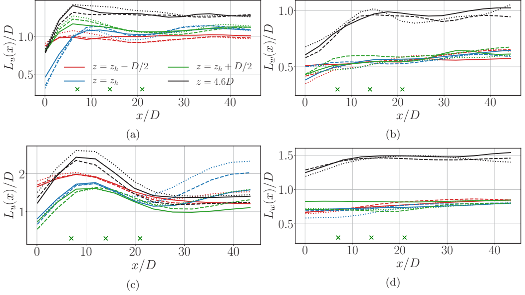
FIG. 13. Moving window correlation-based length scales [Eq. (17)] at different heights for the different cases simulated as in Table III. Solid lines, \lambda_R^3 s_{x,7D} ; dashed lines, \lambda_R^5 s_{x,7D} ; dotted lines, \lambda_R^8 s_{x,7D} . L_u and L_w , length scale based on streamwise and vertical velocity correlation. (a) L_u , window size = 0.2L_x , overlap = 20%. (b) L_w , window size = 0.2L_x , overlap = 20%. (c) L_u , window size = 0.45L_x , overlap = 40%. (d) L_w , window size = 0.45L_x , overlap = 40%. Green crosses denote the streamwise location of the turbine rows.
