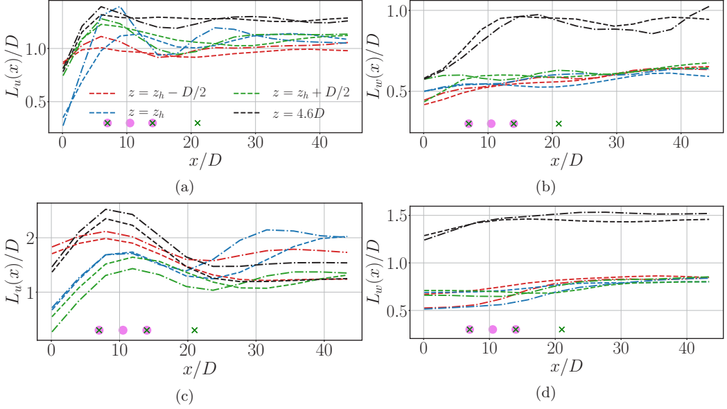
FIG. 14. Moving window correlation-based length scales [Eq. (17)] at different heights for the different cases simulated as in Table III. Dashed lines, \lambda_R^5 s_x, 7D ; dash-dotted lines, \lambda_R^5 s_x, 3.5D . Variable specifications remain the same as in Fig. 13. Green crosses, wind turbine locations with s_x = 7D ; pink circles, wind turbine locations with s_x = 3.5D .
